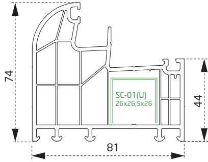
PSC0160BY Kasa Profili Frame Profile
