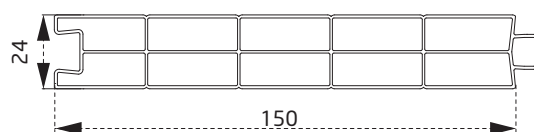
PTS2360BY 24 mm lambri 24 mm paneling
