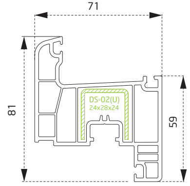
PDR0260BY Kanat Profili Sash Profile
