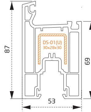
PSY4765BY Kanat Profili Sash Profile
