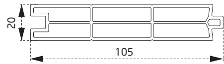
PTS2260BY 20 mm İmbri 20 mm paneling
