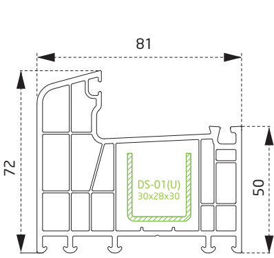
PGR0160BY Kasa Profili Frame Profile
