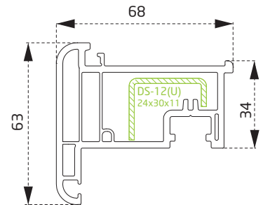
PDR1360BY Stump Profili Stump Profile
